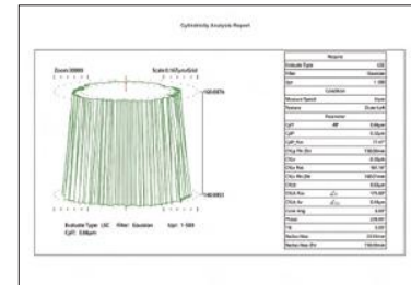
cylindricity analysis
