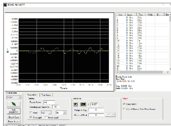
software (included)
