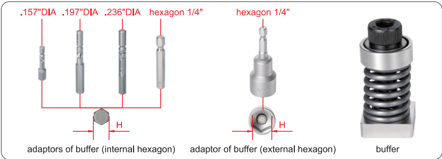
buffer (optional) IST-CD-BF2 type A
