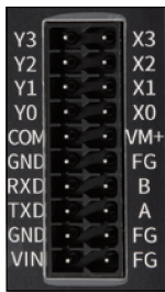
IO output and communication ports (included) type A (side view)
