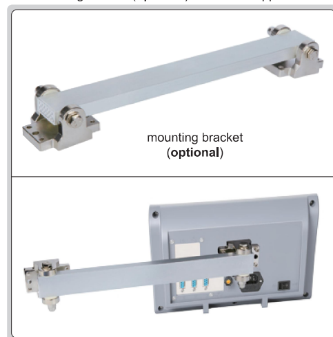
mounting bracket (optional) installation application
