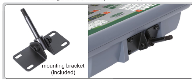
mounting bracket (included) installation application
