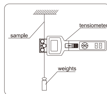
calibration
