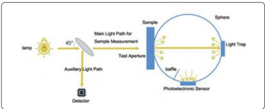
test principle
