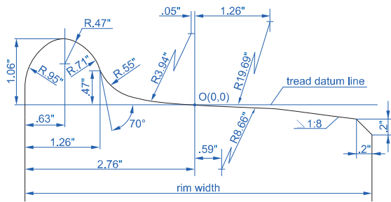
flange and tread contour of 4991-LMT
