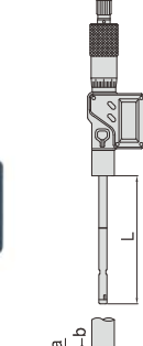
type B .275-.5", steel measuring points
