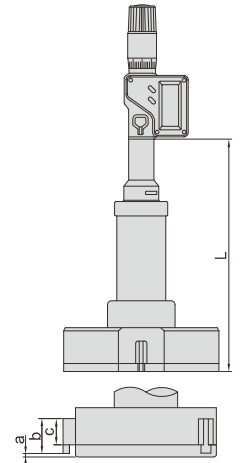
type D 2-12", carbide measuring points
