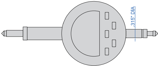
digital indicator
