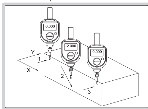
position workpieces
