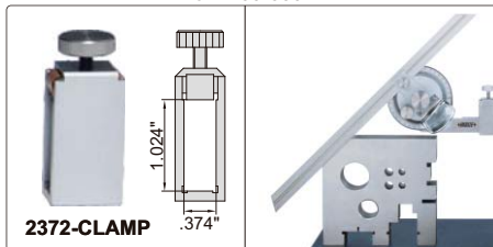
clamp for protractors (optional) for 1150-300E
