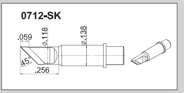
soldering tips (included)
